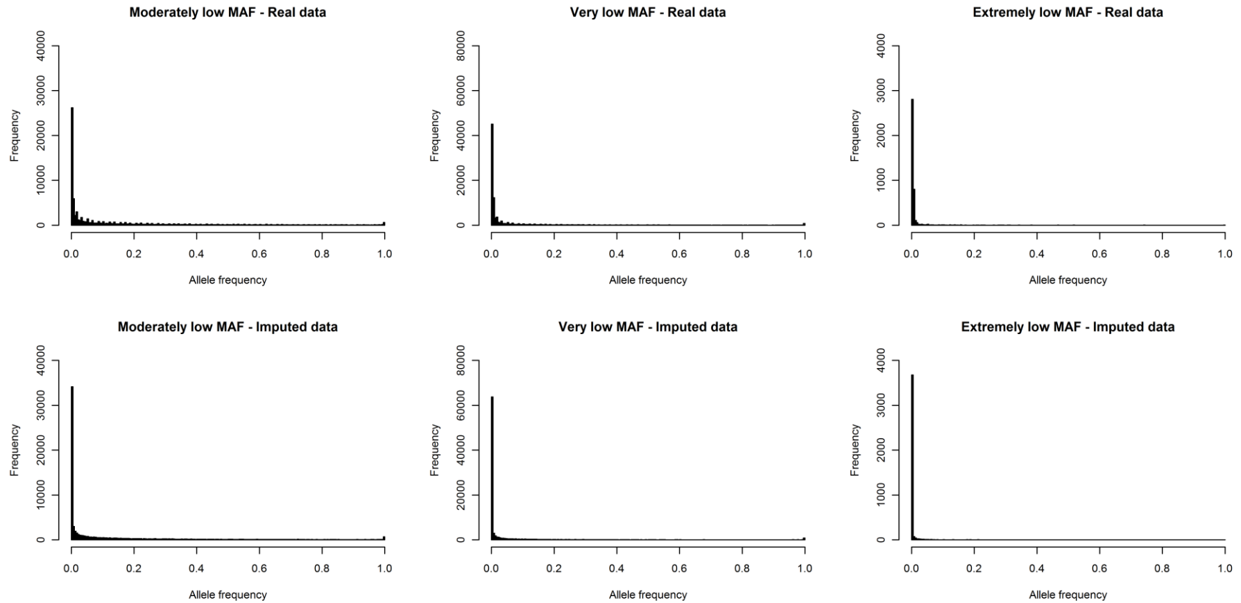
Figure S1 – Allele frequency distribution of imputed and genotyped variants in Holstein Friesian animals. Distribution of allele frequencies of variants with on average a moderately low minor allele frequency (MAF), very low MAF or extremely low MAF in real data and imputed data for Holstein Friesian animals.
