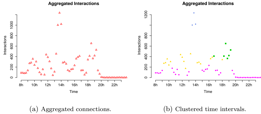
Figure 6: Aggregated connections for each time interval (6a) and time clusters found by our model (6b) are compared.
