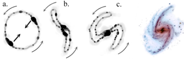
Figure 29: Lathrop hypothesis on Galaxy formation through accretion of dust particles on a vortex ring (a), which gravitate and clump (b) giving the ring a spiral shape (c) and creating the gravitational conditions for the formation of a black hole.
