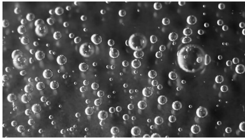
Figure 26: CO 2 bubbles in water representing the concept according to which matter particles, as superfluid vortices in dark energy, create regions where density falls, so the surrounding medium possesses much greater density. The very high value for vacuum energy density deriving from QFT could be then plausible without any cutoff, meaning that what we consider to be “vacuum” owns a much higher energy density than baryon matter itself, albeit not interacting with it as long as the superfluid remains unperturbed.
