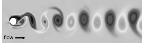
Figure 3: A computer simulation of a Kármán vortex street. Clumps of DEQ (dark matter?) along a flow of superfluid dark energy might be responsible for the appearance of particle-antiparticle pairs as anti-symmetric vortices of DEQ.
