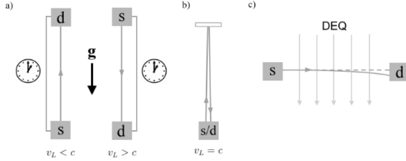
Figure 20: Possible test for verifying superfluid quantum gravity and the photon as a phonon through dark energy. The clocks of source and detector are synchronized to exclude the contribution of gravitational time dilation and the speed of light (or its frequency or wavelength) is measured while it travels up/downward with respect to the gravitational field (a). A slightly lower speed should be detected while light travels upward and, vice versa, light should be faster. The two opposite effects would be balanced in a round trip of light (b) giving v_L = c . On the right (c) SQG too predicts the effect of gravitational lensing due to the gravitational field as a flow of DEQ and to photon as a phonon through dark energy (in the same way wind deflects sound), without resorting to curved space-time.
