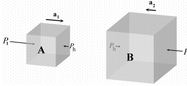
Figure 13: Hydrodynamic representation of gravity in a superfluid flat space. Two bodies attract each other since the vortex-particles which they are constituted of absorb DEQ. The resulting Bernoulli pressures ( P_1 , P_2 ) accelerate A and B the one toward the other, while P_h refers to the homeostatic (internal) pressure of SDE tending to distance all bodies in the SQS (corresponding to \Lambda g_{\mu\nu} in Einstein’s field equations).
