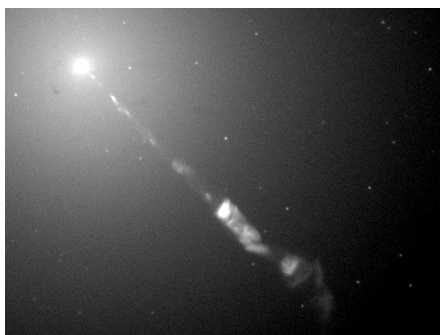
Figure 19: Jet containing gravitationally accelerated ions from the supermassive black hole in Messier 87 (image from the Hubble Space Telescope).
