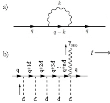
Figure 32: Current (a) and suggested (b) Feynman diagram describing a charged particle's self-energy, where d indicates a quantum of dark energy and \gamma_{\text{DEQ}} a virtual photon as a discrete packet of dark energy quanta.
