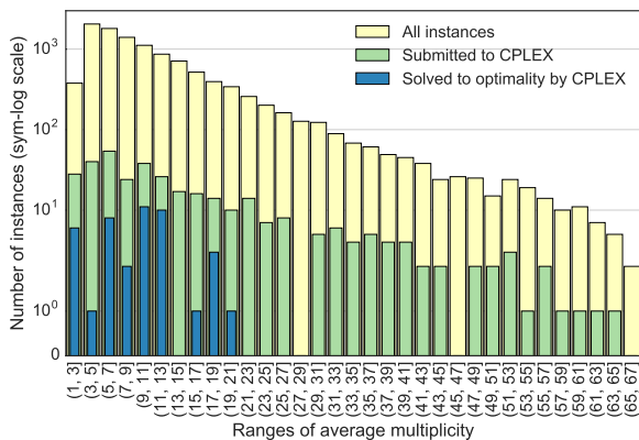
Figure 5: Number of instances by average multiplicity (sym-log scale).
