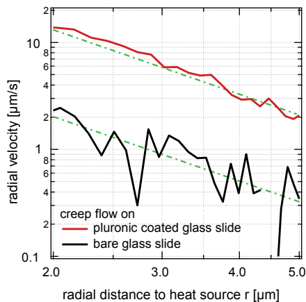
Figure 3. Temperature profile and slip velocity along the upper boundary. The temperature agrees very well the power law \propto r^{-2} . The slip velocity on both glass and Pluronic-coated glass follows this law beyond 2 microns from the heated spot.
