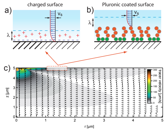
Figure 1. Schematic view of the boundary layer at an interface with non-uniform temperature. a) Thermo-osmotic velocity profile close to a charged solid boundary with an excess enthalpy within an interaction length \lambda ; for z > \lambda the velocity saturates at v_s . b) The same for a Pluronic-coated surface. c) Streamlines in the liquid film resulting from slip velocities at the upper and lower boundaries, reconstructed by numerical calculations and the experimental results for the Pluronic F-127 coated surface.
