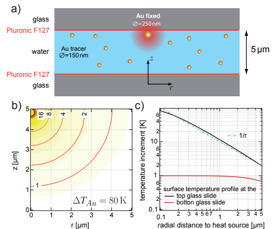
Figure 2. a) Principal design of the experiment. The fluid is contained between two glass cover slides in a sandwich structure with a gap of about 5\mu\text{m} . A R = 125\text{ nm} AuNP is immobilized at the top surface and used as the heat source. A focused laser beam ( \lambda = 532\text{ nm} ) is heating the particle. R = 75\text{ nm} AuNPs were used to measure the velocity field. b) Temperature map around the heated AuNP in cylindrical coordinates r and z . c) Temperature profile along the upper (black curve) and the lower glass (red curve) surface.
