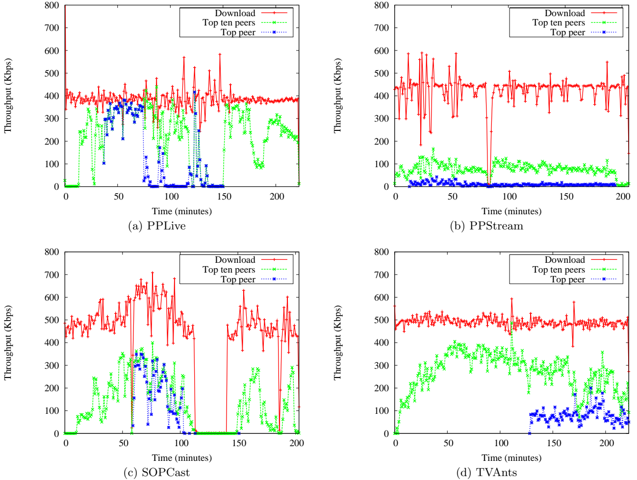
Figure 4: Video download policies: total traffic, top ten peers traffic and top peer traffic. Bin duration is 60s
