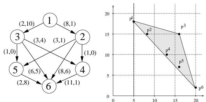
Figure 1: A 2-scenarios problem and its representation
