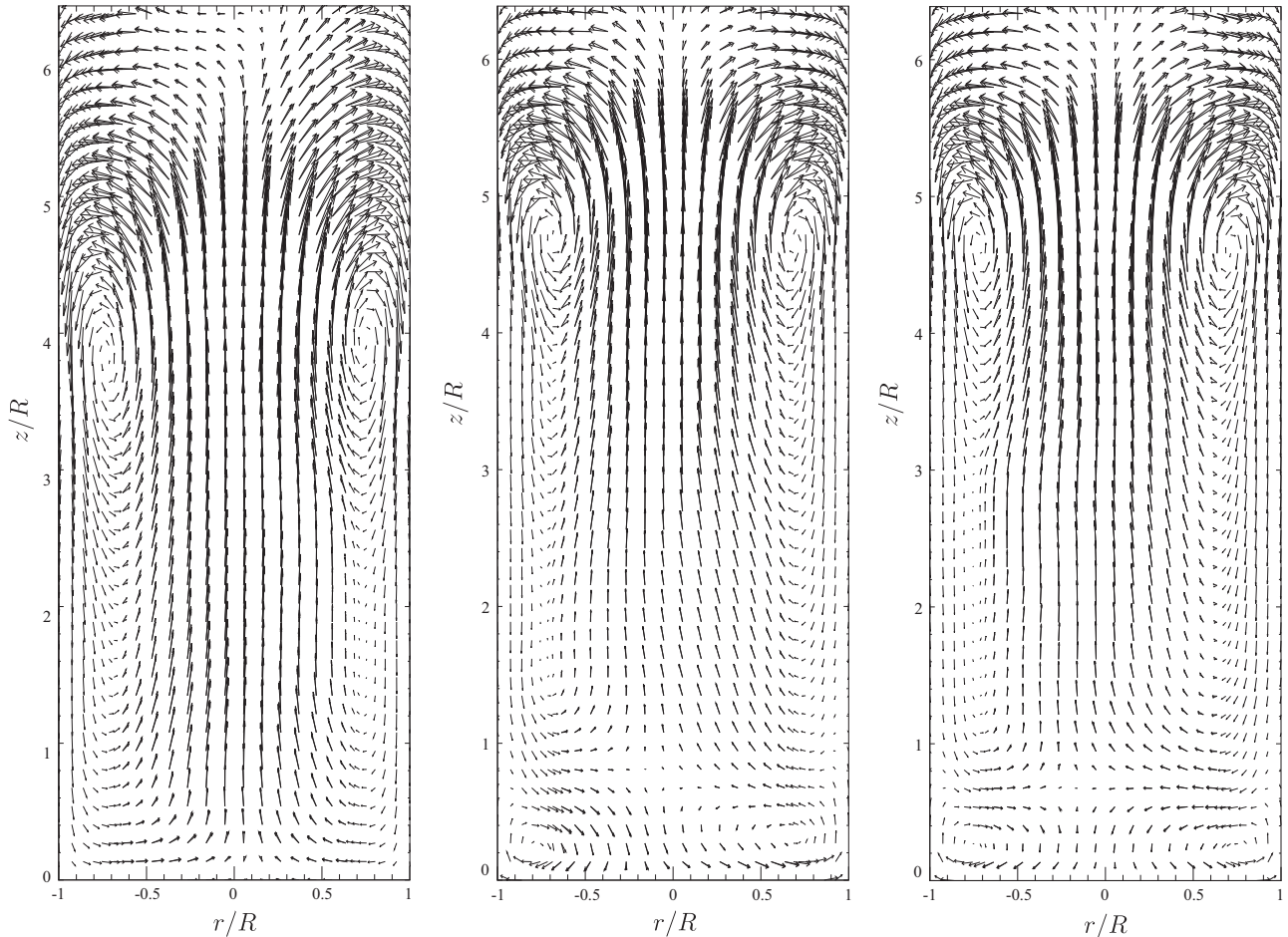
Fig. 8. Effect of the wall boundary conditions for the solid phase on the time-averaged solid velocity field. This vertical plane is passing through the symmetry axis and is defined by y=0 in the simulation mesh. Left: Free-slip, middle: No-slip and right: Johnson and Jackson's rough wall with \phi = 0.1 and e_w = 1.0 boundary conditions for the solid phase.
