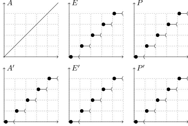
Figure 6: Example of input \langle A, E, P \rangle and output \langle A', E', P' \rangle for a packetizer.
