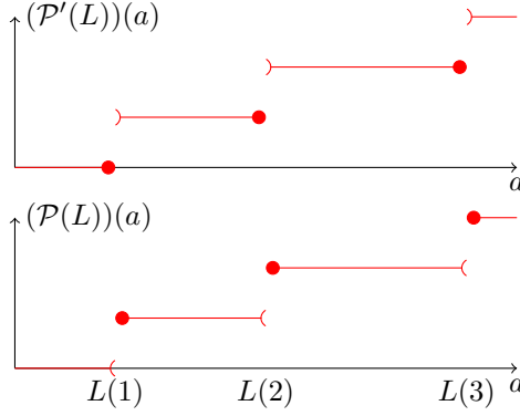
Figure 3: The packet function built from cumulative length.
