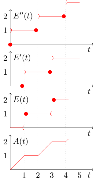
Figure 2: Continuity and packet sizes.
