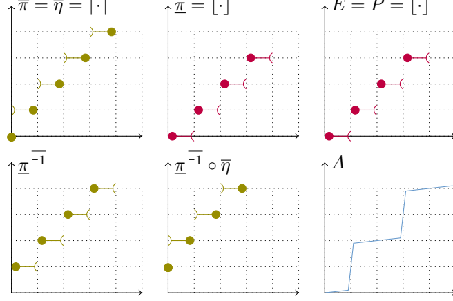
Figure 4: Example of periodic constant size packet.
