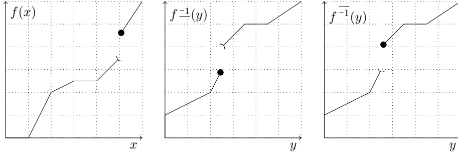
Figure 1: Illustration of pseudo-inverse.
