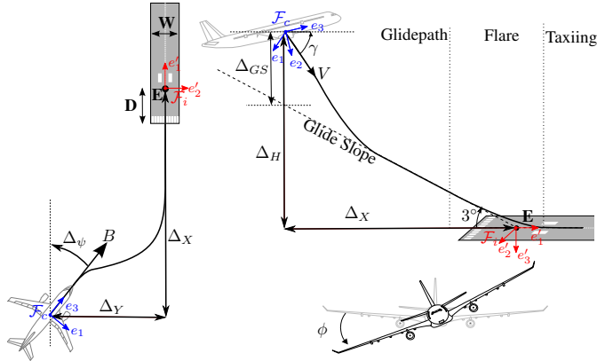
Fig. 1. Notations used in landing phase.
