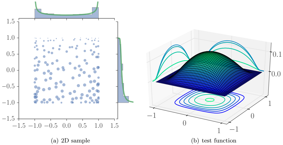
Figure 1: 1(a) A weighted sample of the DPP in Theorem 2.7 with Jacobi base measure, see Section 3 for details. 1(b) The test function (3.1) when d = 2 .
