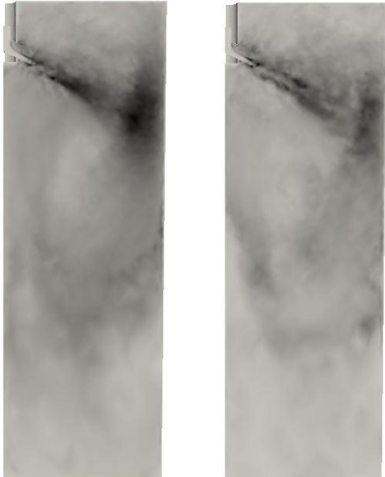
Figure 4: Velocity standard deviation with no EMS (left) and with EMS (right)
