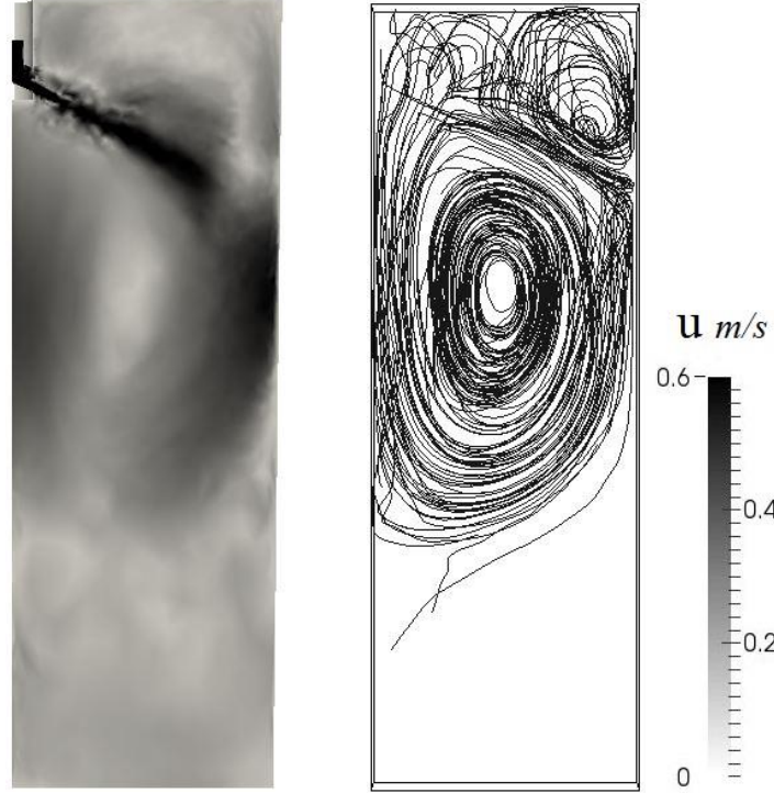
Figure 3: Averaged velocity magnitude (left) and streamlines in the double-roll area (right)
