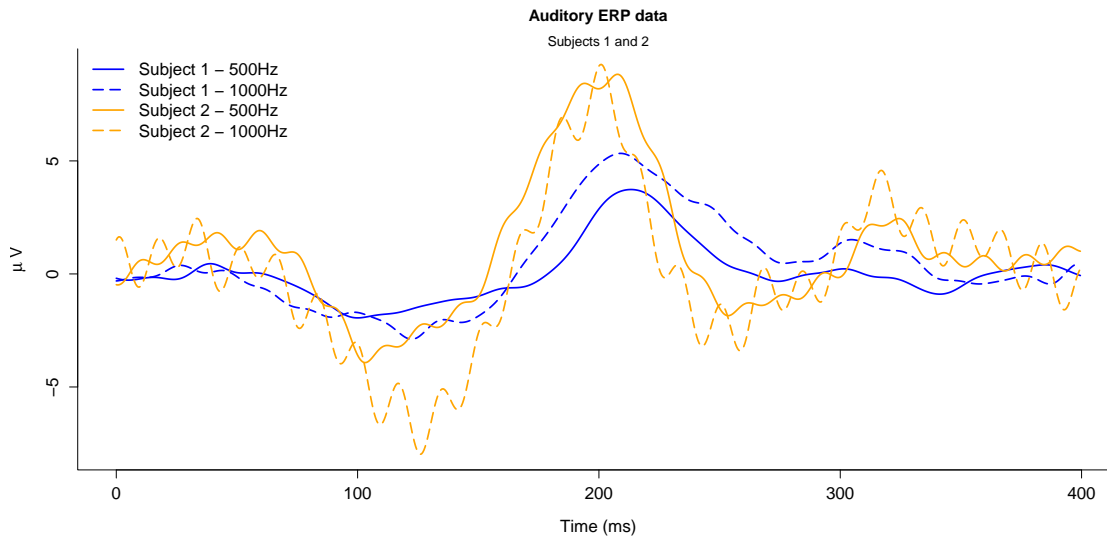
Figure 1: ERP curves for subjects 1 (blue lines) and 2 (orange lines) of the auditory oddball experiment in conditions Hz500 (plain) and Hz1000 (dashed)
