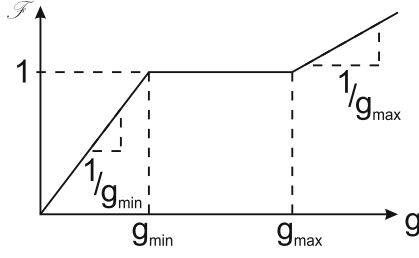
Fig. 6 Value of \mathcal{F} versus the penetration
