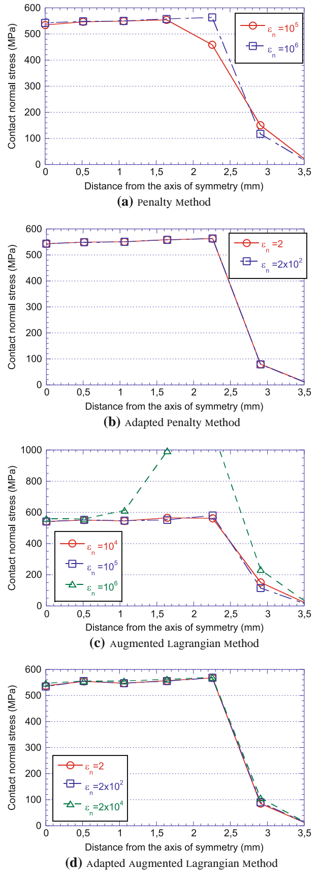
Fig. 17 Contact normal stress (mesh 4; elastoplastic problem)
