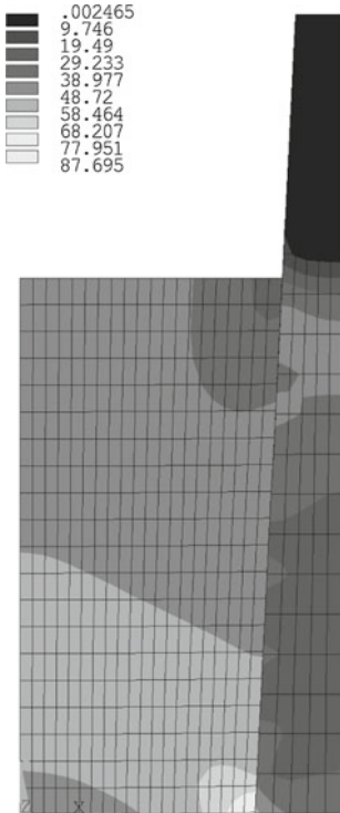
Fig. 22 von Mises stress distribution (MPa, PM with \varepsilon_n = 10^4 and \varepsilon_t = 10 )
