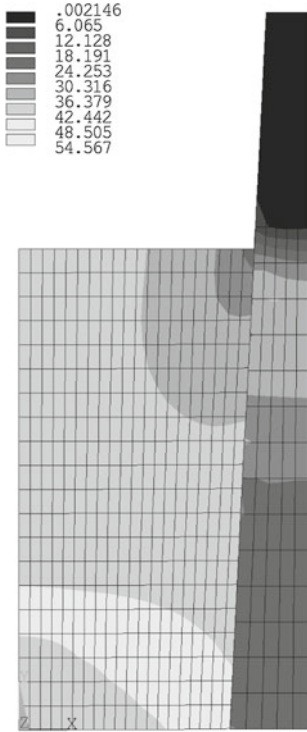
Fig. 21 von Mises stress distribution (MPa, PM with \varepsilon_n = 10^3 and \varepsilon_t = 1 )
