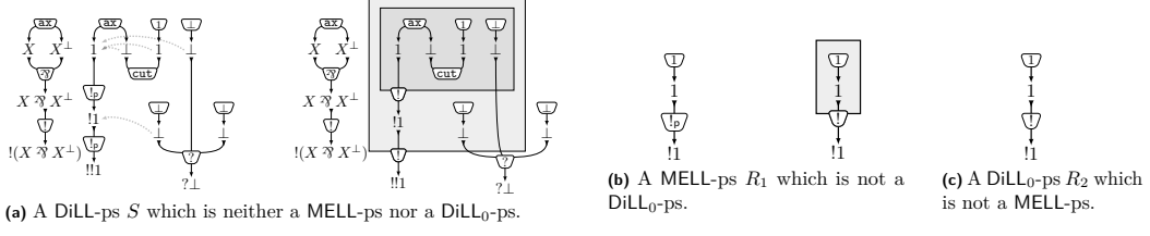
■ Figure 3 Some examples of DiLL-ps. In R_1 (Fig. 3b) \mathcal{C}_{R_1}^{\text{box}} = \{l\} and \text{box}_{R_1} is the empty function. In R_2 (Fig. 3c) \mathcal{C}_{R_2}^{\text{box}} = \emptyset , so \text{box}_{R_2} is the empty function. Both S (Fig. 3a) and R_1 (Fig. 3b) are in two different presentations: the “arrow-like” one (on the left) and the “inductive-like” one (on the right).
