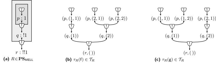
■ Figure 7 A MELL-ps R (Fig. 7a, where o and l are the box -cells with conclusion of type !1 and !!1 , respectively), and two different but isomorphic elements \tau_R(f) (Fig. 7b) and \tau_R(g) (Fig. 7c) of \mathcal{T}_R , where f and g are the Taylor-functions of R defined in Example 33.
