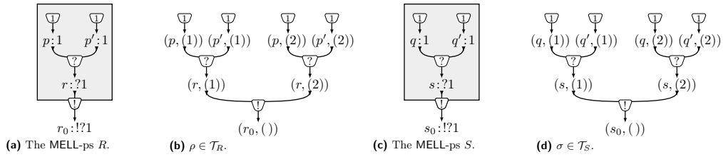
■ Figure 11 Two box-connected and isomorphic MELL-ps R and S (where \mathcal{C}_R^{\text{box}} = \{l\} and \mathcal{C}_S^{\text{box}} = \{o\} ), with \rho \in \mathcal{T}_R and \sigma \in \mathcal{T}_S strongly fat.
