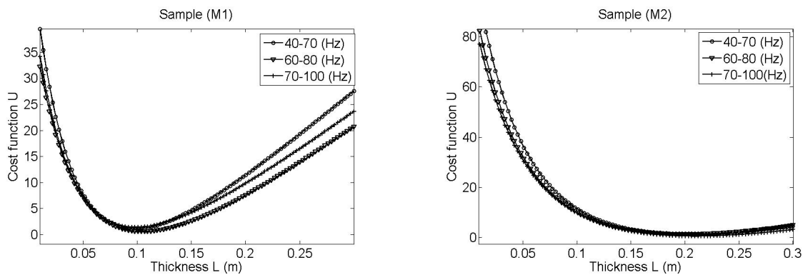
Figure 7 - Variation of the minimization function U with thickness L of samples M1 and M2
