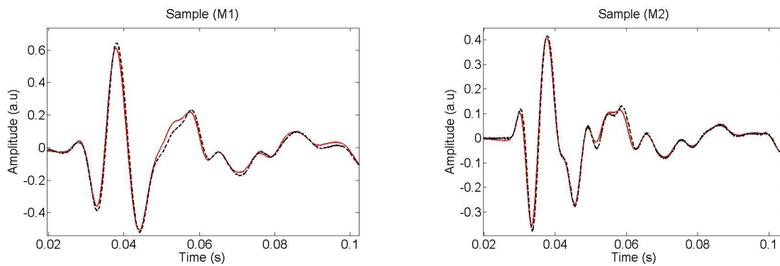
Figure 5. – (Color online) Comparison between the experimental transmitted signal (dashed line) and the simulated transmitted signals (solid line) using the reconstructed values of \sigma of samples M1 and M2
