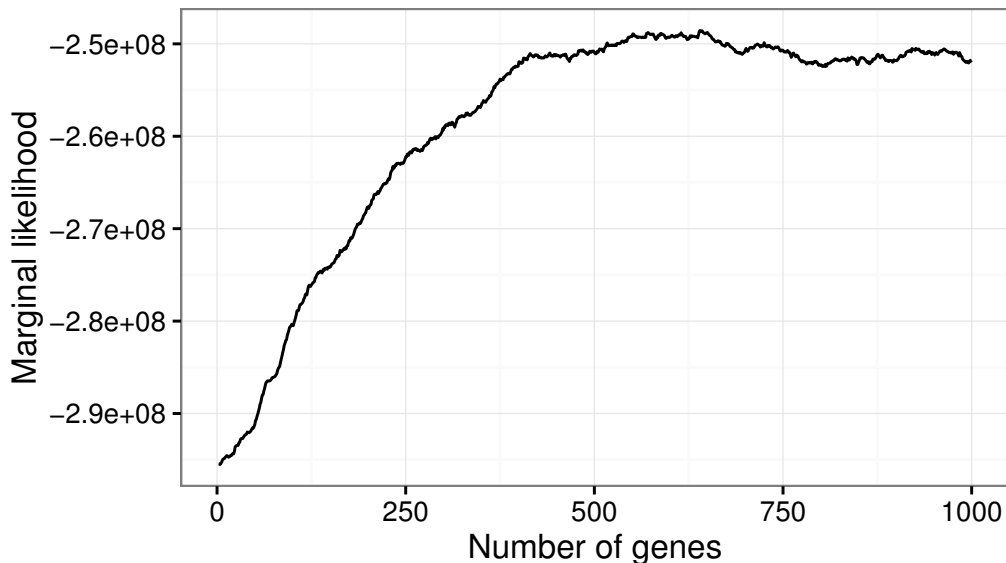
Figure 5: Marginal likelihood for the gene selection problem
