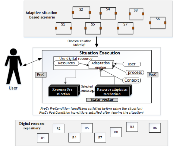
Fig. 1. Digital resource management architecture
