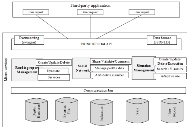
Fig. 4. PRISE API REST-based micro-services architecture
