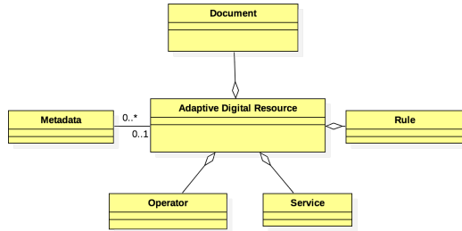
Fig. 2. Adaptive Digital Resource diagram class
