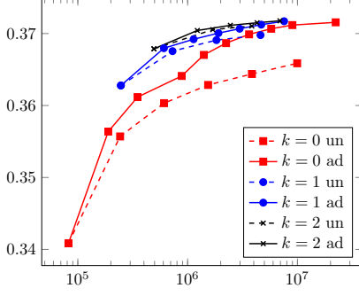
(a) Capacitance vs. N_{\text{dof}}
