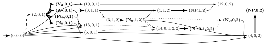
Fig. 5. Hypergraph representing the chart parsing of the substring set points with the FSSA from Fig. 3. The double, plain, thick, dashed, densely dotted and loosely dotted hyperarcs represent axioms, pseudo substitution, deactivate, scan, foot adjoin and root adjoin inference rules, respectively (see Sec. 4.4). Passive states are highlighted in bold.
