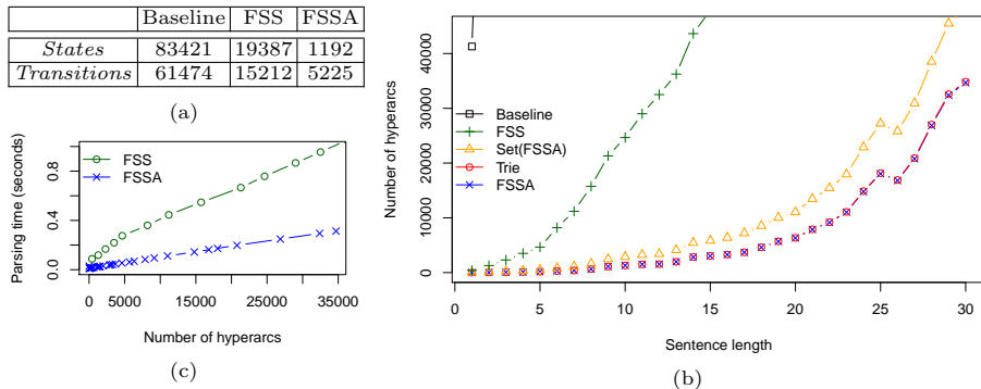
Fig. 6. (a) Results of the compression experiments, (b) Impact of grammar encoding methods on parsing performance, measured as an average number of hyperarcs explored by the parser on \sim 13000 sentences randomly generated from the FrenchTAG grammar, (c) Average parsing time as a function of the number of generated hyperarcs.
