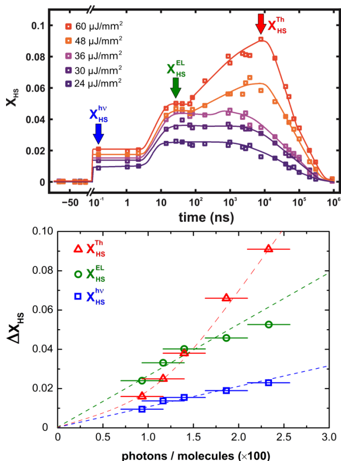
Figure 4. a) Response to femtosecond laser excitation of LS [\text{Fe}(\text{Phen})_2(\text{NCS})_2] at 140 K for different excitation densities "hv", "El" and "Th" denote respectively the photoinduced, elastic and thermal steps. b) Evolution of X_{\text{HS}}^{\text{hv}} (measured at 10 ps) scaling with the number of incident photon per 100 molecules. On the photo-switching step \approx 1 molecule is transformed per photon, whereas on the elastic step ( X_{\text{HS}}^{\text{El}} ) \approx 2.5 -3 molecules are transformed per photon. Heating effect appears at high excitation density (close to sample damage).
