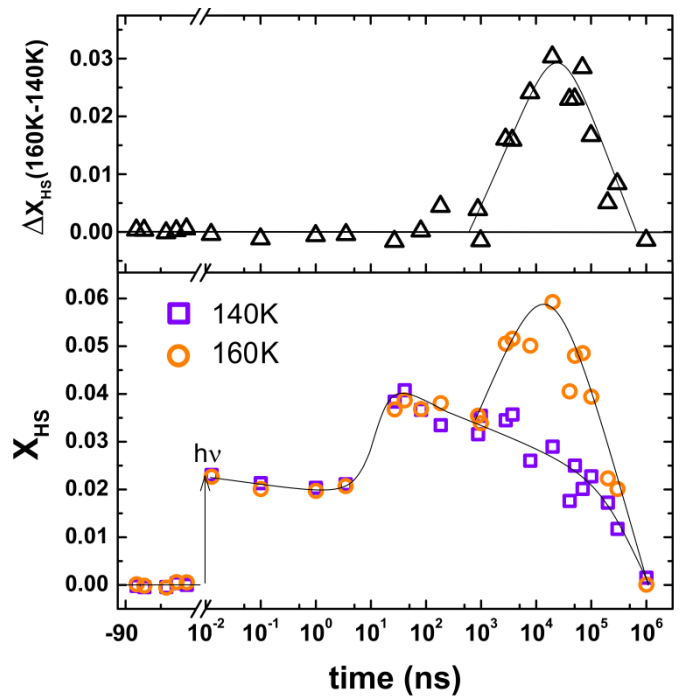
Figure 6. Evolution of the HS fraction X_{\text{HS}} after femtosecond laser excitation of LS [\text{Fe}(\text{Phen})_2(\text{NCS})_2] at 140 and 160 K for 30 \mu\text{J}/\text{mm}^2 excitation density.
