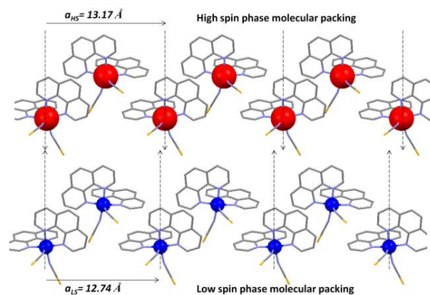
Figure 3. The molecular swelling between LS and HS states induces lattice expansion, shown in along the a crystalline axis.
