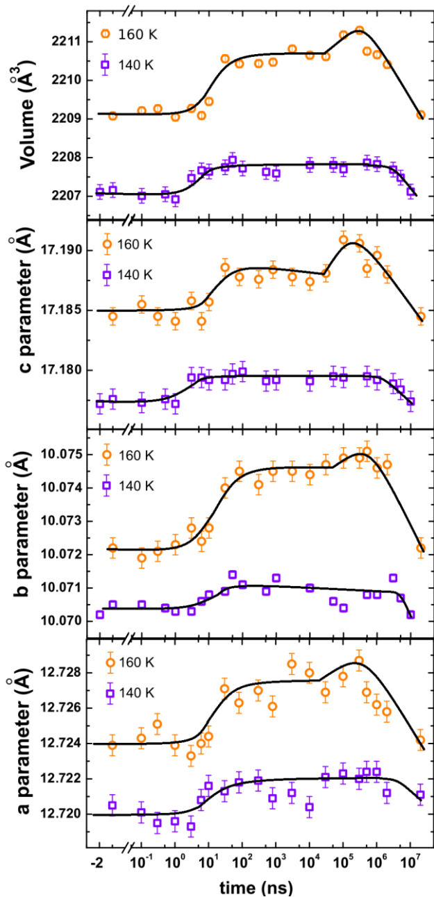
Figure 5. a) Lattice response to femtosecond laser excitation of LS [\text{Fe}(\text{Phen})_2(\text{NCS})_2] at 140 K for an excitation density of 20 \mu\text{J}/\text{mm}^2 and at 160 K for an excitation density of 30 \mu\text{J}/\text{mm}^2 .
