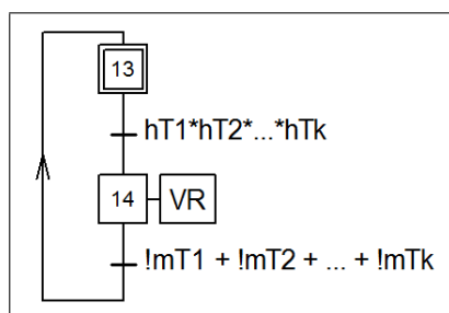
Figure 5. Grafset specification of opening/closing the exhaust valve VR .
