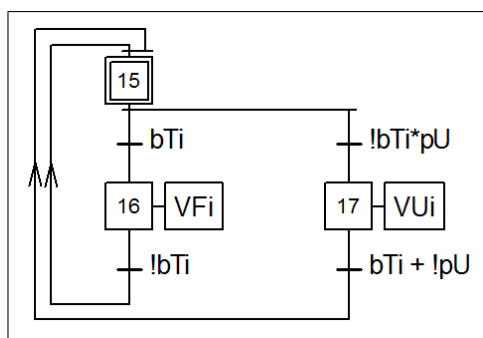
Figure 6. Grafset specification of water providing floors
