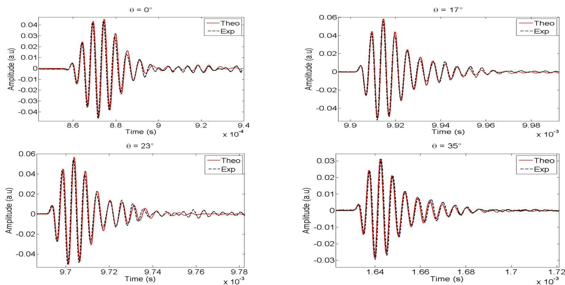
Fig.4 Comparison between experimental reflected signal (dashed line) and simulated reflected signal (solid line) for the plastic foam sample M ( \theta_0 = 0^\circ, 17^\circ, 23^\circ and 35^\circ )
