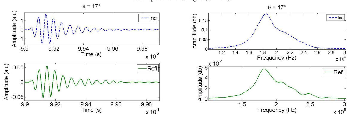
Fig.3(b)- Experimental incident signal (dashed line) and experimental reflected signal (solid line) at left and their spectrum at right ( \theta = 17^\circ ).
