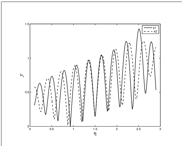
Figure 4. Mono-frequency mismatch functions \mathcal{F} (see Eq.(15)) for k_1 = 10 and k_2 = 11 , \theta = \pi , the target is an ellipsoid of semi-axis (1.0 – 1.5). On can observe that the only minimum location that doesn't change when the frequency of the mismatch function change is the expected solution ( \rho = 1.5 in this case).
