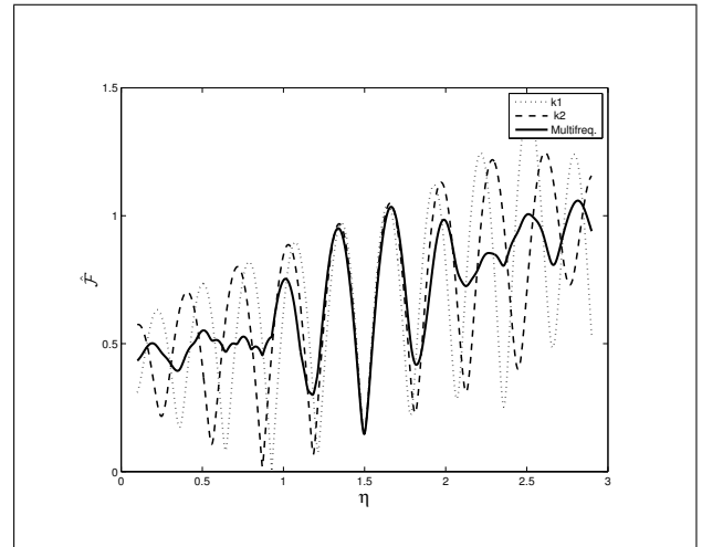
Figure 5. Same as Figure(4) but the plot of the multifrequency cost function is added (see Eq.(16): M=4 , k_1 = 8 , k_2 = 9 , k_3 = 10 , k_4 = 11 ). One observes that the "multifrequency" cost function admits a global minimum at the expected position ( \rho = 1.5 ).
