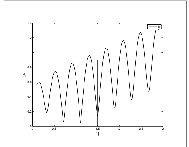
Figure 2. see Eq.(15)) for k = 8, \theta = \pi, r_b = 3 , the target is an ellipsoid of semi-axis (1.0 - 1.5) . One can observe the presence of local minima: the expected solution ( \eta = 1.5 ) is not the global one ( \eta = 1.1 ). The vertical straight line indicates the expected location of the solution.
