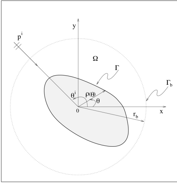
Figure 1. Scattering configuration.
