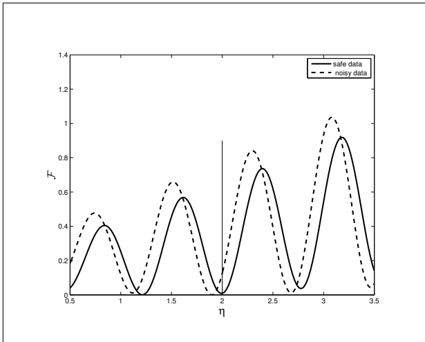
Figure 3. see Eq.(15)) for k = 4 , \theta = \pi , r_b = 6 , the target is an ellipsoid of semi-axis (1.5 – 2). One can observe the displacements of the locations of the minima when adding noise to the data. The vertical straight line indicates the expected location of the solution.
