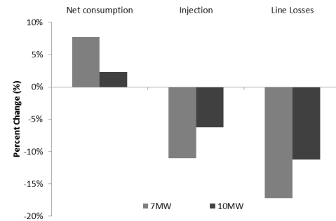
Fig. 4. Percentage increase or decrease due to added storage elements at each PV production node. Calculations for a 7 MW and 10 MW systems during a three days period using typical summer profiles
