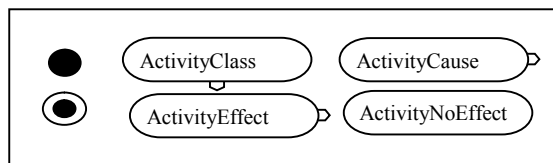
Figure 4. ActivityModule components.
