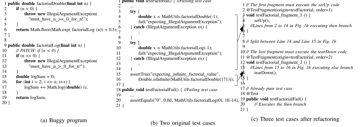
Fig. 1: Example of refactoring a test suite. The buggy program and test cases are extracted from Apache Commons Math. The buggy if is at Line 11 of Fig. 1a. A test case testFactorial in Fig. 1b executes both then (at Line 10 of Fig. 1b) and else (at Line 15 of Fig. 1b) branches of the if (at Line 11 of Fig. 1a). Fig. 1c shows the test cases after the splitting (between Lines 14 and 15) according to the execution on branches.
