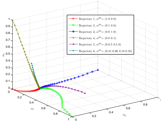
Fig. 3. Trajectories of the Krasonsielkij algorithm with different starting points all converging to the same WE \alpha^* = (0.61, 0.17, 0.18, 0.02) . The settings for this simulation is: U_0^\gamma = 0 ; U_1^\gamma = \gamma(3 - 2\alpha_1 - \alpha_2 - \alpha_3) - 1.5 ; U_2^\gamma = \gamma(3.5 - 1.5\alpha_2 - 0.75\alpha_1 - 0.75\alpha_3) - 2 ; U_3^\gamma = \gamma(4.5 - 2\alpha_3 - \alpha_1 - \alpha_2) - 3 . Notice that the value of \alpha_0 is not reported in axes of the figure since \sum_{c \in C} \alpha_c = 1 .
