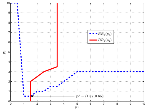
Fig. 4. Best-responses lines for a network where 2 NSPs offering one service each. Each leader estimates the WE of the users' game and evaluates its own optimal price for each of the possible price taken by the other leader. The meeting point of the two lines is the (unique) NE.
