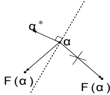
Fig. 1. Geometrical interpretation of condition (17). The distance between F(\alpha) and \alpha^* might be bigger than the distance between \alpha and \alpha^* . However, the angle between the vectors F(\alpha) - \alpha and \alpha^* - \alpha is minor than \frac{\pi}{2} .
