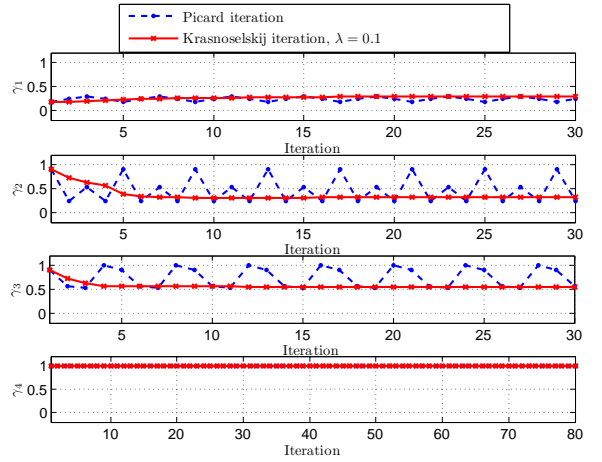
Fig. 2. Thresholds as functions of iteration steps. The dashed line marked with circles represents the evolution of the thresholds when all the users best-respond and are allowed to change their strategy, whereas the continuous line marked with crosses represents the evolution of the thresholds when a fraction equal to \lambda = 0.1 of users is allowed to switch their strategy. Note that, in the fourth plot, the two lines are superposed.
