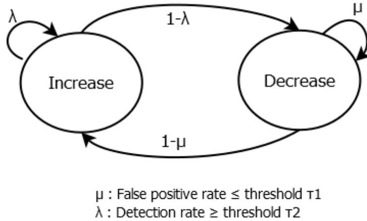
Figure 5: Stochastic timer update process.
