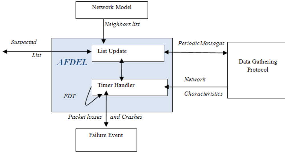
Figure 2: Interactions between AFDEL and system modules.
