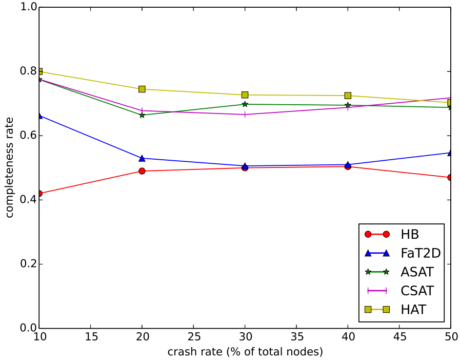
Figure 7: Completeness evaluation VS number of crashes (scenario2).
