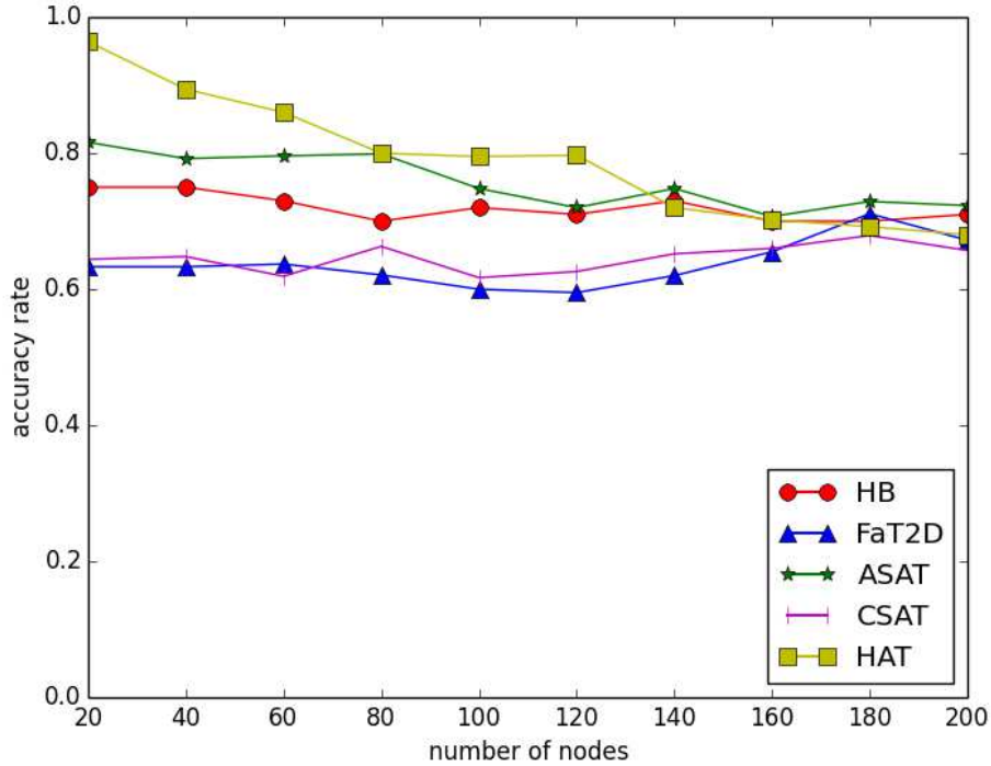
Figure 8: Accuracy evaluation VS number of nodes (scenario1).
