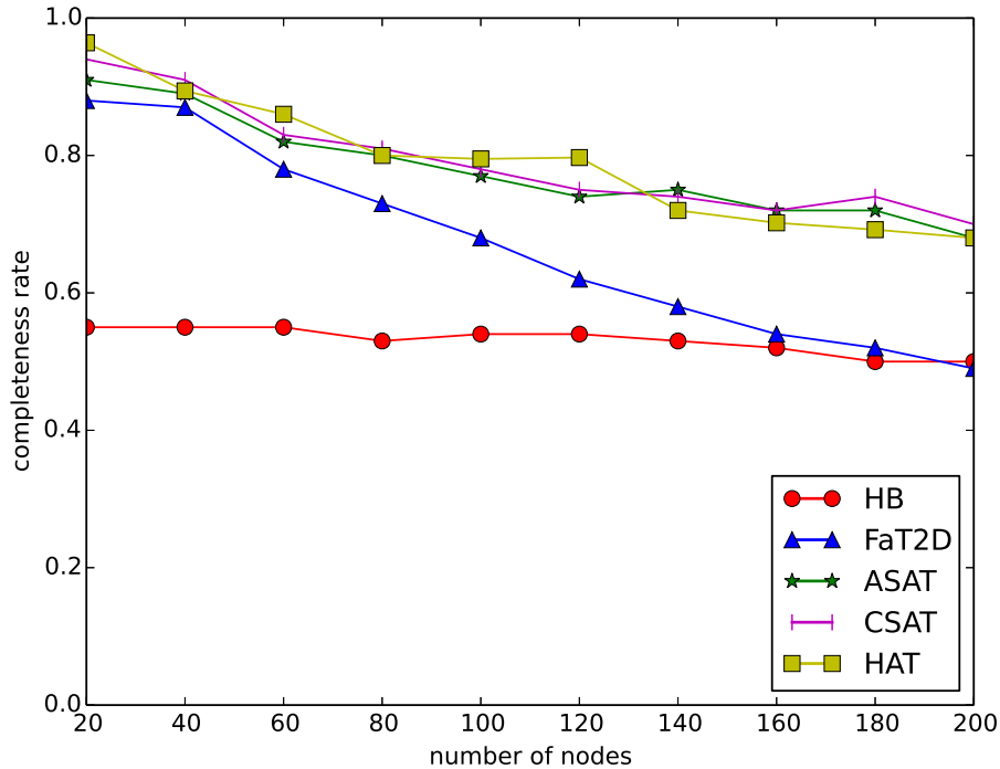
Figure 6: Completeness evaluation VS number of nodes (scenario1).
