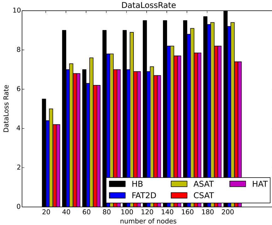
Figure 11: Data Loss Rate.
