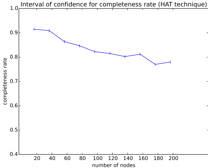
Figure 14: Confidence Interval for completeness rate (HAT technique).
