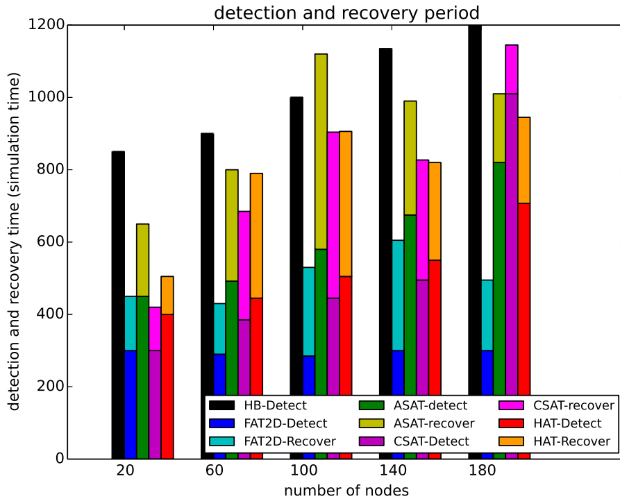
Figure 10: Detection and Recovery time.
