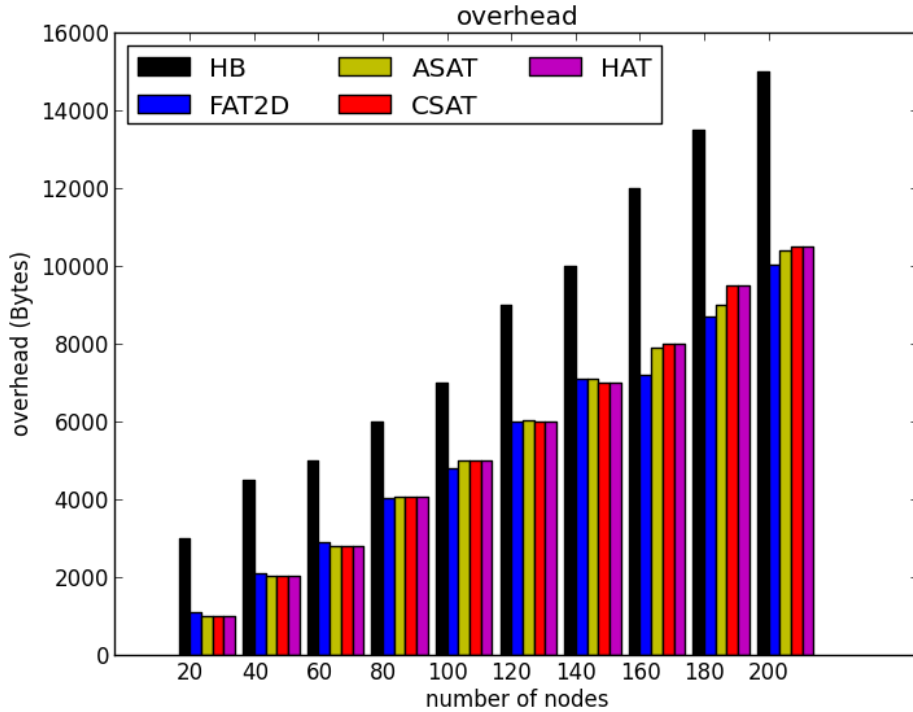
Figure 13: Overhead evaluation.
