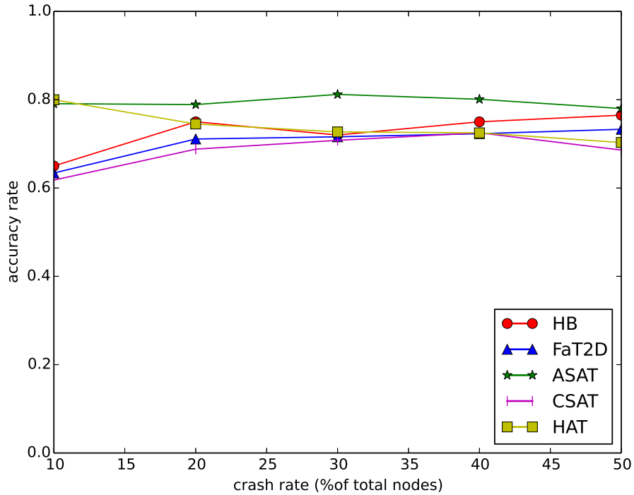
Figure 9: Accuracy evaluation VS number of crashes (scenario2).
