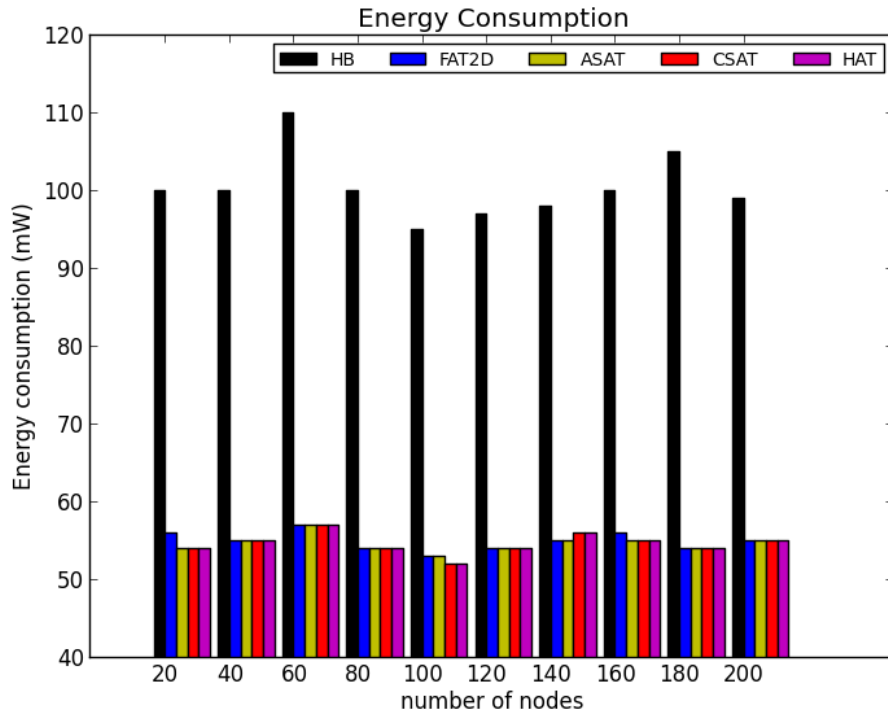
Figure 12: Performance of energy consumption.
