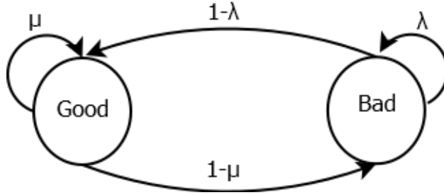
Figure 1: Gilbert-Elliott packet loss model.
