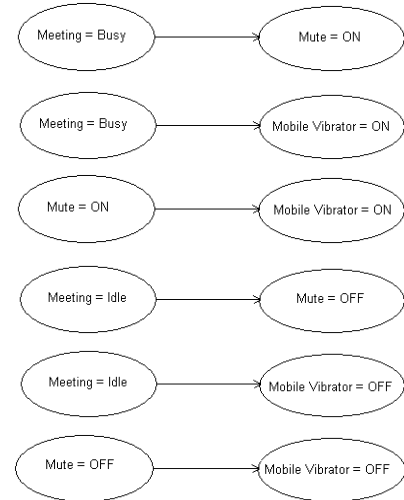
Fig. 6 Dependency Graph
