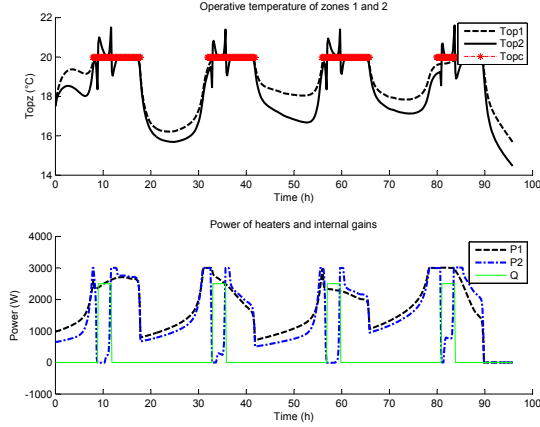
Figure 2 – Optimal command and temperature response
