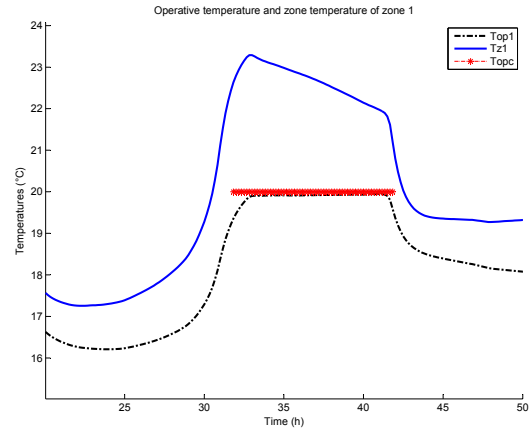
Figure 4 – Comparison between zone 1 temperature and corresponding operative temperature
