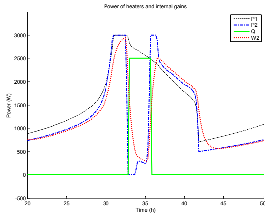
Figure 3 – Optimal command : Non controlled gains compensation
