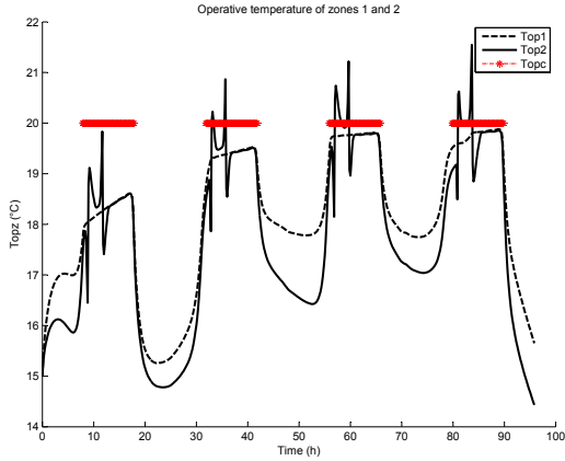
Figure 8 – Temperature response with a bias of 1.5^\circ\text{C} on initial temperatures
