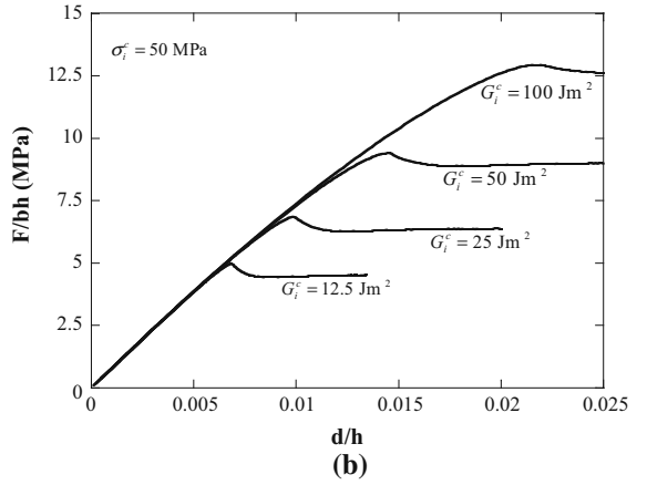
Fig. 7 Predictions provided by the bilinear CZM : a crack length and b load-displacement curve versus the applied displacement for \sigma_i^c = 50 MPa and various values of G_i^c
