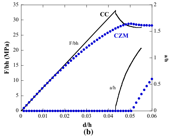
Fig. 9 Comparison between the load-displacement and crack-displacement response predicted by CC and bilinear CZM: a \sigma_i^c = 100 MPa, G_i^c = 50 Jm -2 , b \sigma_i^c = 100 MPa, G_i^c = 500 Jm -2
