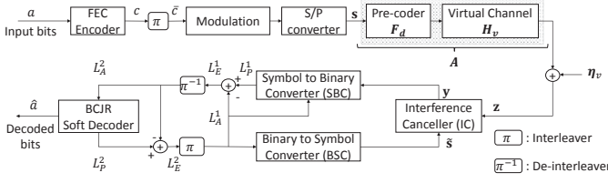
Fig. 1: Equivalent system model.
