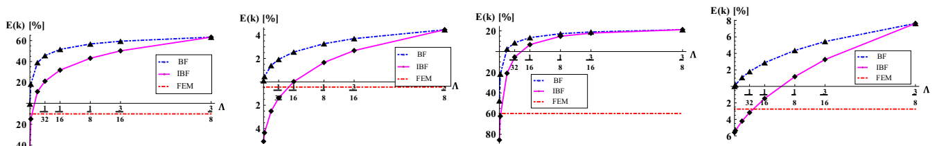
FIG. 28. (Color online) This figure shows the Darcy-Brinkman zone \sigma = 1520 , R_B = \frac{k_B}{k_D} \approx 0.92 (2D), and R_B \approx 0.8 (ML1).
