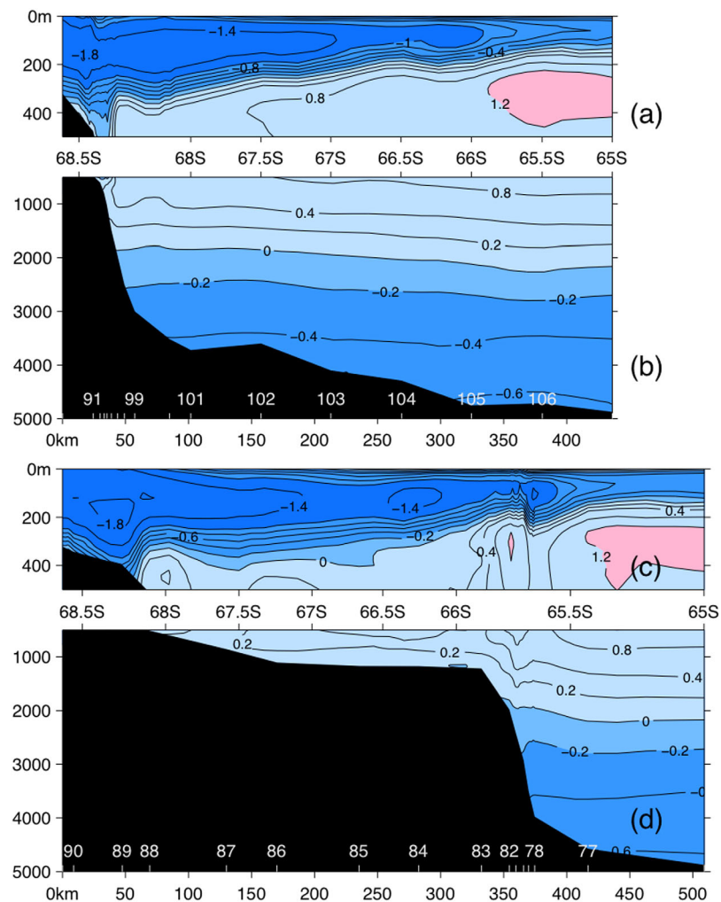
Figure 3. Potential temperature ( ^{\circ}\text{C} ) of the western section (STATIONS 91-106-76; a and b) and the eastern section (STATIONS 76-90; c and d) from CTD data. The upper 500 m in both sections are stretched to show more details (a and c). Selected station numbers are shown at the bottom (b and d).
