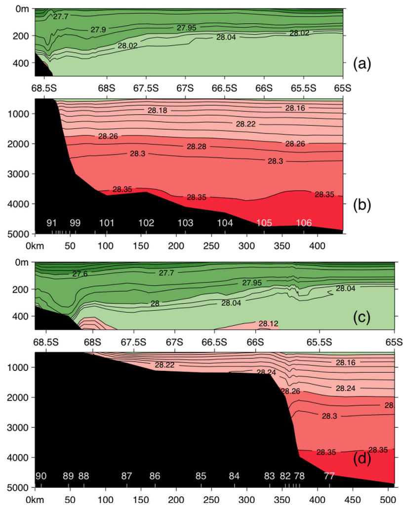
Figure 5. Neutral density ( \text{kg/m}^3 ) of the western section and the eastern section as in Figure 3.
