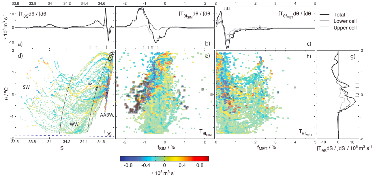
Figure 2. Overview of residual volume transports across the combined ANDREX-I6S section. (a) Residual volume transports as a function of S class. Black, dark gray, and light gray lines, respectively, refer to the total, lower cell, and upper cell flows. The small arrows at the base of the panel indicate residual-transport-weighted-mean S values, with the same color coding as the lines. Solid and dashed arrows are associated with inflows and outflows, respectively. (b) Residual volume transports as a function of f_{SIM} class. Lines and arrows follow the convention in Figure 2a. (c) Residual volume transports as a function of f_{MET} class. Lines and arrows follow the convention in Figure 2a. (d) Residual volume transport in \theta - S space (in bins of 0.01^\circ\text{C} ( \theta ) and 0.0025 ( S )). The residual-transport-weighted-mean \theta - S coordinates of the inflows and outflows are indicated by solid and dashed symbols, respectively. The coordinates associated with the total flow are marked by squares, and those associated with individual overturning cells are marked by circles. As in Figures 1b and 1c, isopycnals separating major water masses are indicated by black contours, and those marking the transport maxima of and the boundary between the gyre's two overturning cells are shown by (dashed) gray contours. The freezing point of seawater is shown by the black dashed line. (e) Residual volume transport in \theta - f_{SIM} space (in bins of 0.01^\circ\text{C} ( \theta ) and 0.025\% ( f_{SIM} )). The area corresponding to the lower cell is indicated by hatching. (f) Residual volume transport in \theta - f_{MET} space (in bins of 0.01^\circ\text{C} ( \theta ) and 0.025\% ( f_{MET} )). The area corresponding to the lower cell is indicated by hatching. (g) Residual volume transports as a function of \theta class. Lines and arrows follow the convention in Figure 2a.
