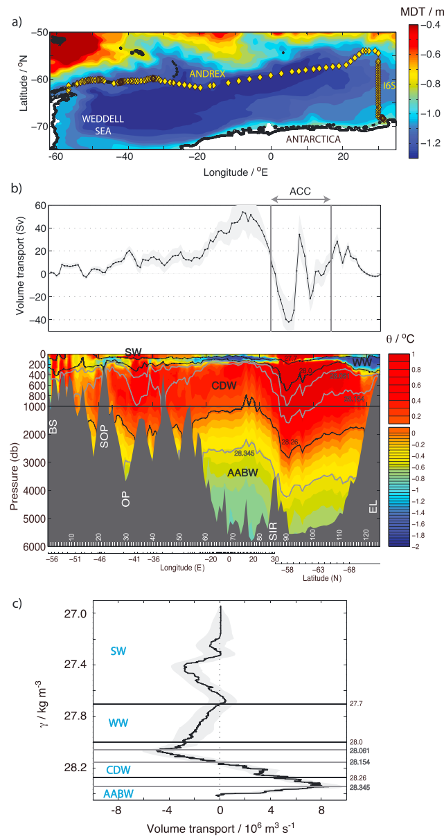
Figure 1. Overview of the setting and results of the Weddell Gyre inverse model of Jullion et al. [2014]. (a) Map of the ANDREX and I6S stations (diamonds). The (2005–2010 time-averaged) mean dynamic topography in the Southern Ocean State Estimate [Mazloff et al. , 2010] is shown by the background shading. (b) top: full-depth volume transport across the combined ANDREX-I6S section (positive transport directed out of the gyre). The uncertainty is indicated in gray, and the segment of the section within the ACC is marked on the upper axis. bottom: vertical section of potential temperature (color) and selected neutral density surfaces (contours), with station number (labeled in white) as the horizontal axis. Isopycnals separating major water masses (SW = surface waters; WW = Winter Water; CDW = Circumpolar Deep Water; AABW = Antarctic Bottom Water) are indicated by black contours and labels, and those marking the transport maxima of and the boundary between the gyre’s two overturning cells are shown by gray contours and labels. The following topographic features are indicated: Bransfield Strait (BS), EL (Enderby Land), OP (Orkney Passage), SOP (South Orkney Plateau). (c) Accumulated volume transport across the combined ANDREX-I6S section, with water masses and isopycnals indicated as in Figure 1b. The uncertainty is shown in gray.
