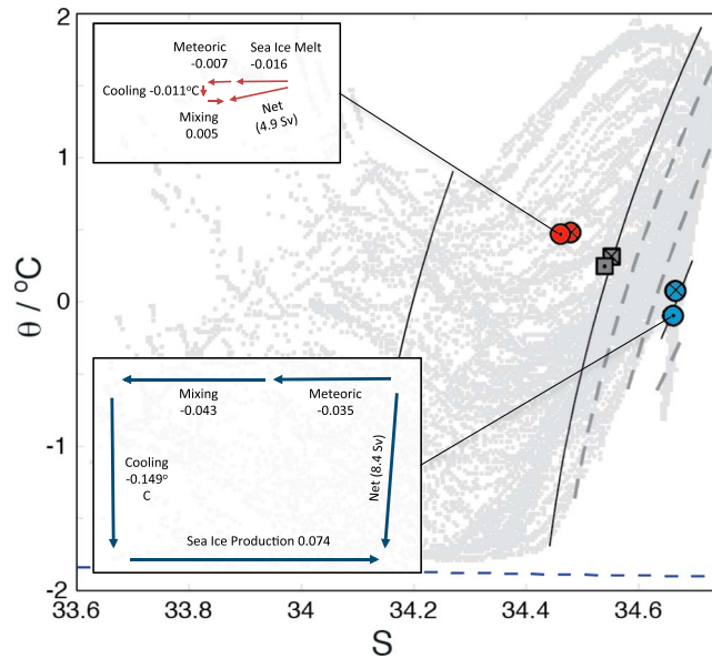
Figure 3. Schematic synthesis of the thermodynamic balance of the Weddell Gyre. The gray shading indicates the area of \theta - S space occupied by water masses along the rim of the gyre. The residual-transport-weighted-mean \theta - S coordinates of the inflows and outflows are indicated by the crossed and dotted symbols, respectively (total flow in gray, upper overturning cell in red, lower overturning cell in blue). As in Figures 1b and 1c, isopycnals separating major water masses are indicated by black contours, and those marking the transport maxima of and the boundary between the gyre's two overturning cells are shown by (dashed) gray contours. The freezing point of seawater is shown by the black dashed line. The insets show the changes in \theta and S associated with individual thermodynamic drivers for each of the overturning cells, where the term "mixing" refers to exchanges of WW and CDW between the two cells. Arrow lengths are approximately scaled by the represented change in \theta or S , and arrow widths by the volume transport of the pertinent overturning cell (denoted in brackets next to the net \theta - S transformation).
