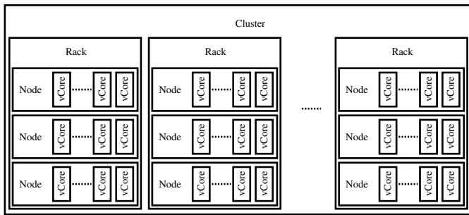
Fig. 1. Hadoop cluster
