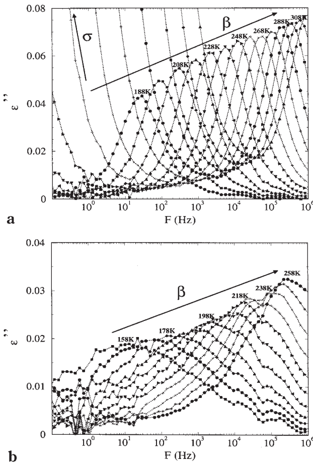
Figure 2. (a) Frequency and temperature dependence of the dielectric energy loss for the \beta -mode of [G_0] . (b) Frequency and temperature dependence of the dielectric energy loss for the \beta -mode of [G_2] .
