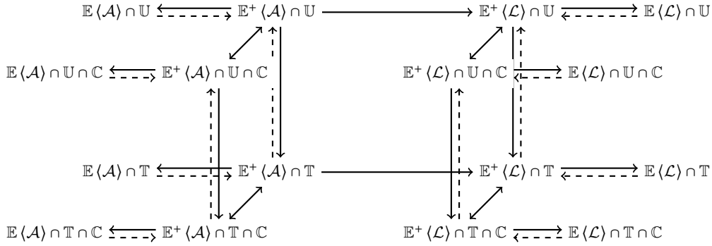
■ Figure 1 The two cubes as sets
