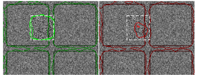
FIG. 5: Four contours with increasing time (black to light) for the (LL) method (left) and the (HD) method (right). The initial contour is on a grid of large squares. For (LL) the contour converges towards the target area T_1 (white dashed line). For the (HD) method the contour shrinks down to a point (divergence).
