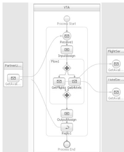
Figure 2: Service orchestration
