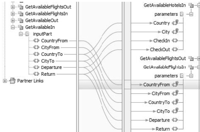
Figure 3: Input merging in service composition
