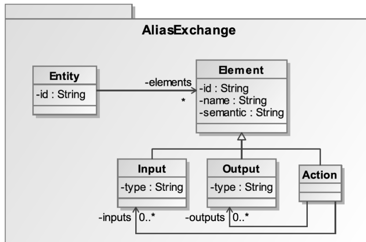
Figure 5: AliasExchange Metamodel
