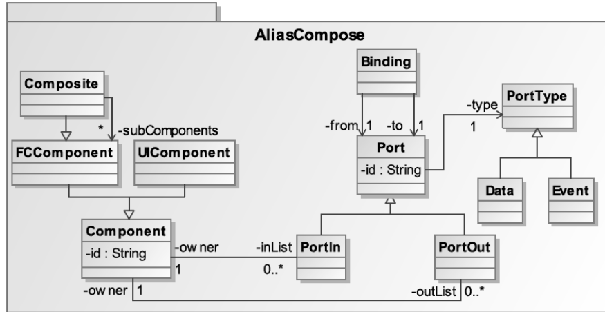
Figure 8: AliasCompose Metamodel
