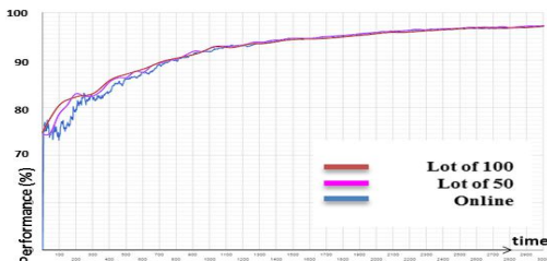
Figure 2. Online and batch mode (ORHD Dataset)
