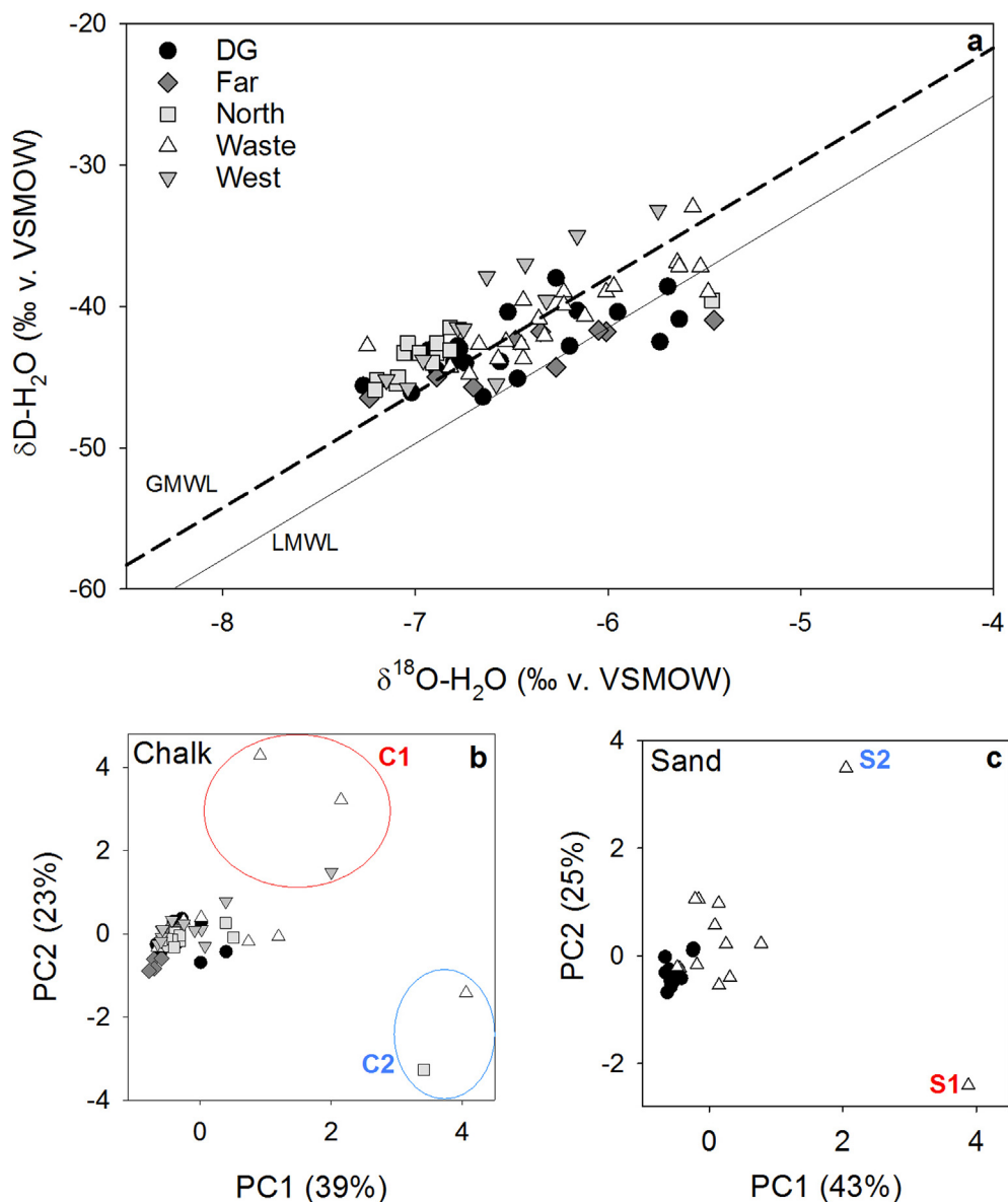
Fig. 2. The isotopic (a) and chemical (b,c) composition of groundwater in a shallow sand aquifer ( n = 24 ) and the deeper, confined chalk aquifer ( n = 40 ) underlying an industrial site in eastern Belgium. In (b) and (c) the PCA of groundwater chemistry are projected onto axes for the first two PCs, and percentage of variance explained noted on their respective axes. Outlier values are labelled S1 (red) and S2 (blue) in sand, C1 (red) and C2 (blue) in chalk. Axes in (b) describe 58% (x) and 29% (y) of variance, and were primarily driven by \text{HCO}_3^- , \text{Mg}^{2+} , and \text{K}^+ . Axes in (c) describe 43% (x; primarily driven by \text{K}^+ , \text{Na}^+ , and \text{HCO}_3^- ) and 25% (y; primarily driven by \text{Cl}^- and \text{Mg}^{2+} ) of variance. (For interpretation of the references to colour in this figure legend, the reader is referred to the web version of this article.)
