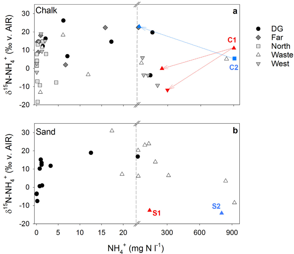
Fig. 4. Relationship between \text{NH}_4^+ concentration and isotopic composition within the chalk (a) and sand (b) aquifers underlying an industrial site in eastern Belgium. Samples were collected from 70 locations directly under the site (light colours: North, Waste, West) and further downgradient (dark colours: DG, Far). Hypothesised contaminant source locations indicated with red (S1, C1) and blue (S2, C2) symbols, with arrows between points indicating regional flow direction. Note change in x-axis scale after 25 \text{mg N l}^{-1} . (For interpretation of the references to colour in this figure legend, the reader is referred to the web version of this article.)
