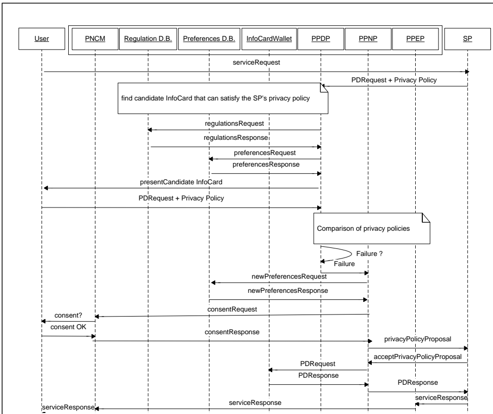
Fig. 5. Sequence Diagram of Data Flows between the User and the SP
