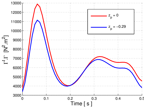
Figure 9: Quadratic torque
