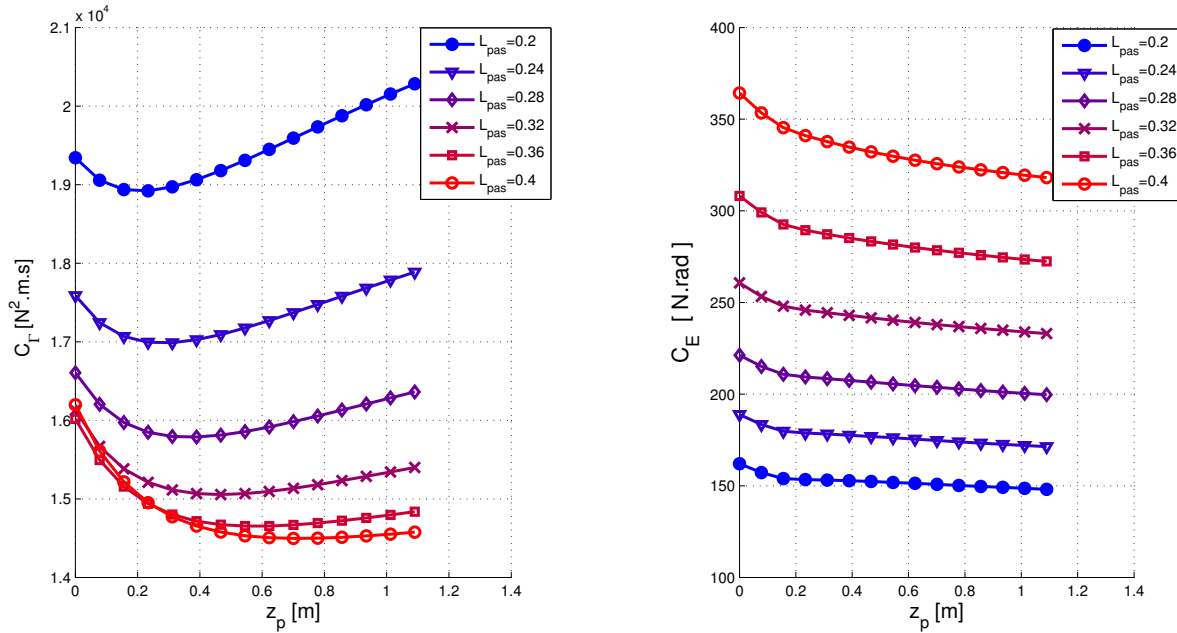
Figure 12: Sthenic criterion as a function of step size. Figure 13: Energy criterion as a function of step size.
