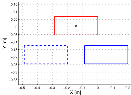
Figure 3: Feet placement for motion planning. The projection of the pivot point in the horizontal plane is represented by the black asterisk.
