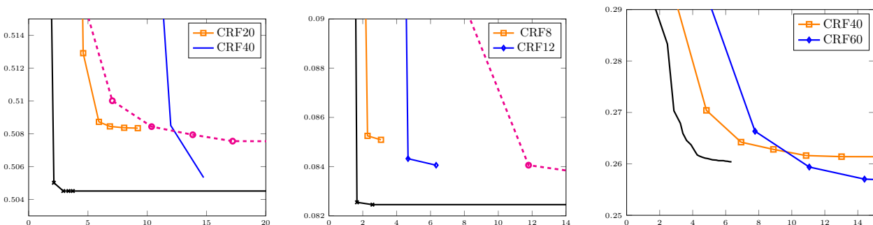
Figure 4: Mumford-Shah energy at time t (in seconds) divided by the same energy for the best constant image obtained with: Non-convex relaxation ( TV_{0.5} - -○- ), \ell_0 cut pursuit ( \ell_0 -CP) -×- and \alpha -expansions (CRFi), for the Shepp-Logan phantom (left), our simulated example (middle) and the map simplification (right). Markers corresponds respectively to one reweighting, one \alpha -expansion cycle and one cut for ( TV_{0.5} ), (CRF) and ( \ell_0 -CP).
