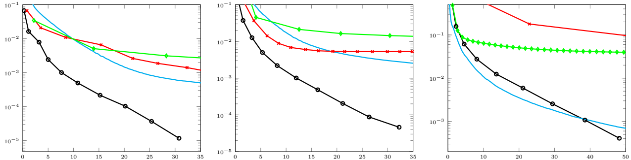
Figure 3: Relative primal suboptimality gap Q_t/Q_\infty - 1 at time t (in seconds) for different algorithms on the deblurring task: FB+: —◆— , PGFB: —■— , CP: —○— , CPFW: —×— , for three 512 \times 512 images and different regularization values: Shepp-Logan phantom (left), our simulated example (middle) and Lena (right). Each marker corresponds to a cut computation for CP, CPFW, and a proximal operator computation for FB+.
