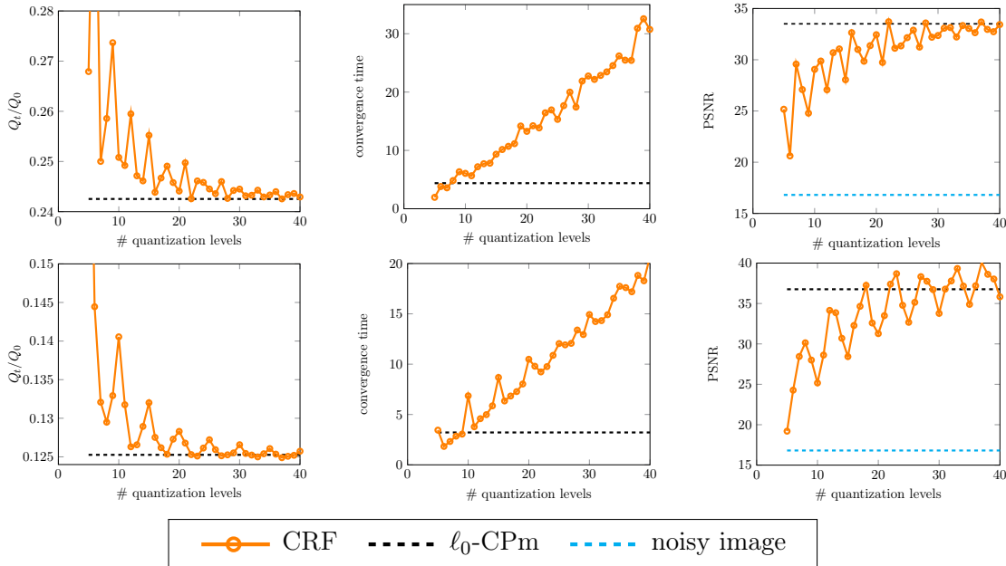
Figure 14: Behavior of the \alpha -expansion based algorithm on CRF formulations for different number of quantization levels for the phantom (top) and the simulated data (bottom) averaged on 10 denoising experiments: (left) ratio between the energy Q at convergence and the energy at time 0, (middle) running time, (right) corresponding PSNRs. The two algorithms represented are \alpha -expansions (CRF) for a varying number of quantization levels and \ell_0 -CPm.
