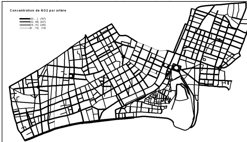
Fig. 6. Network branches and NO 2 concentration
