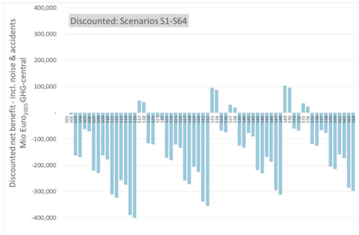
Figure 46: Discounted results of costs and benefits regarding internal and external costs for power plant and passenger cars of scenario S1- 64 compared to the reference scenario S1 (including greenhouse gases based on central value for GHG valuation, air pollutants, noise & accidents; accounting for costs of ETS certificates for the power plants) – [million €2005 ]
