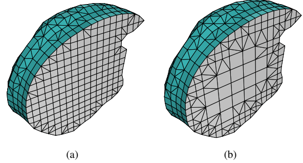
Figure 4. Using surface and transition patterns: (a) regular tongue mesh including only surface patterns, i.e., the ROI is the entire domain, (b) non-regular tongue mesh including surface and transition patterns, i.e., the ROI is limited to the set of octants intersecting the input surface.
