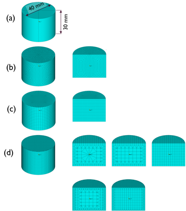
Figure 2. (a) Cylindrical specimen modeled for the FEA of the semi-confined compression test, (b) full tetrahedral mesh, (c) full hexahedral mesh and (d) mixed-element meshes.
